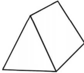
triangular prism
