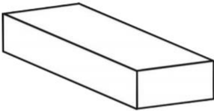
cuboid
